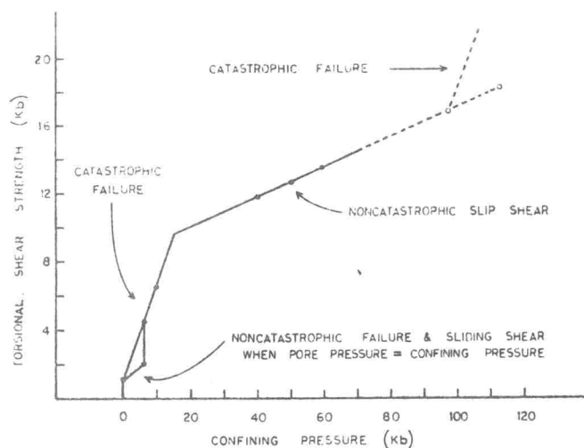
Fig. 1. The postulated failure diagram for normally brittle plutonic rock given by Giardini [1969].
