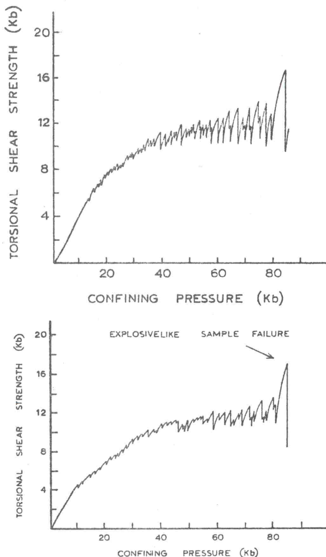
Fig. 2. (Top) The room temperature shear strength of granodiorite obtained with the Abey-Stromberg apparatus using dual disk-shaped samples 1.27 cm in diameter and 0.25 cm high. The samples were subjected to 11^\circ of applied twist at a rate of 10^{-4} rad s^{-1} concurrent with a linearly increasing confining pressure to 85 kbar. The experiment was terminated short of an explosivelike failure of the rock. (Bottom) The room temperature torsional shear strength of granodiorite to about 85 kbar of linearly increasing pressure with 22^\circ of twist concurrently applied at a rate of 10^{-4} rad s^{-1} . Here one of the dual-disk-shaped samples underwent explosivelike failure at about 85 kbar of confining pressure. Shear strength values along the irregular part of this curve and other shear strength curves given in this paper refer to maximums along the curves.
